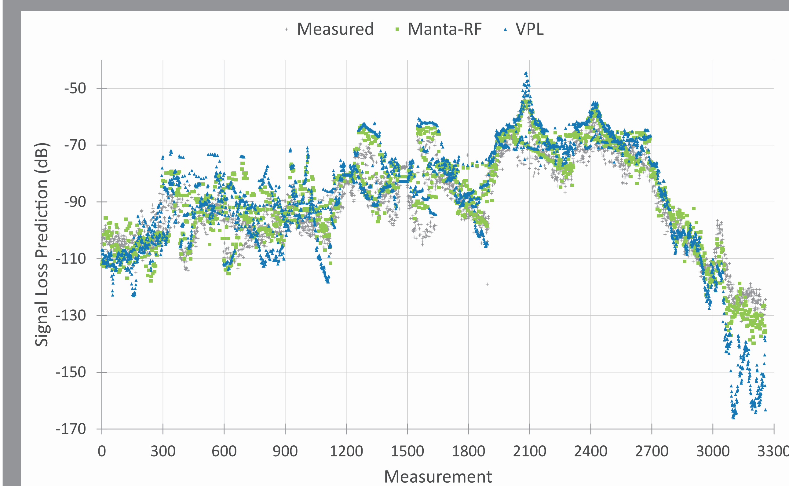
Comparison of signal loss predictions using Manta-RF and VPL [Liang & Bertoni 1997] against measured data from the Rosslyn, VA dataset (measurement locations shown at left).
